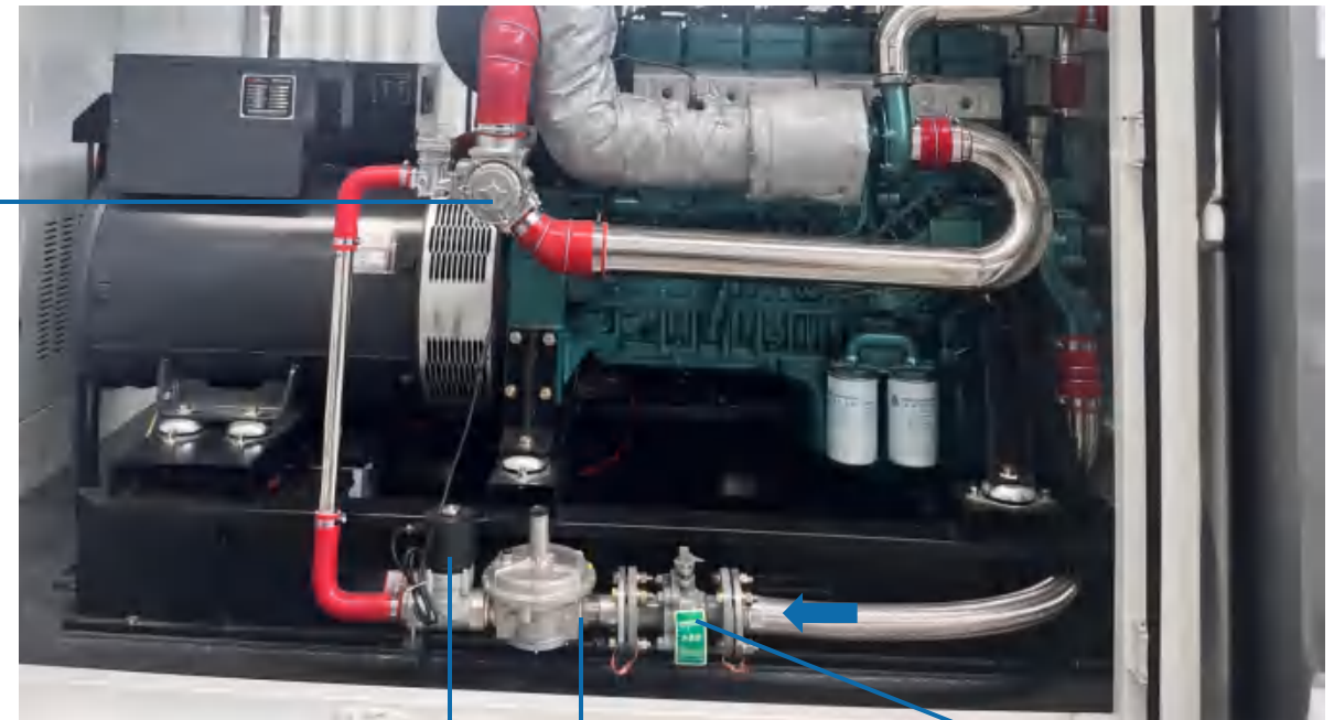
Pressure regulator
