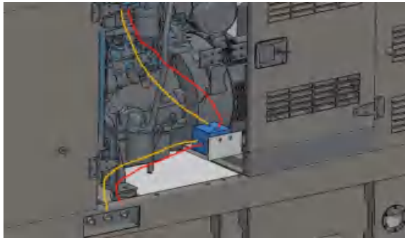
3-way valve external cabling
