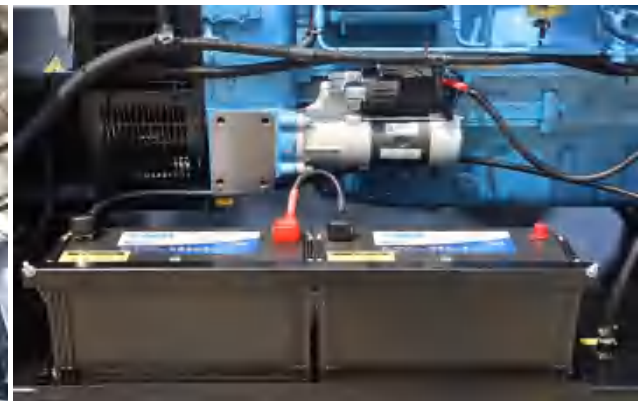
Acrylic electrical protection
